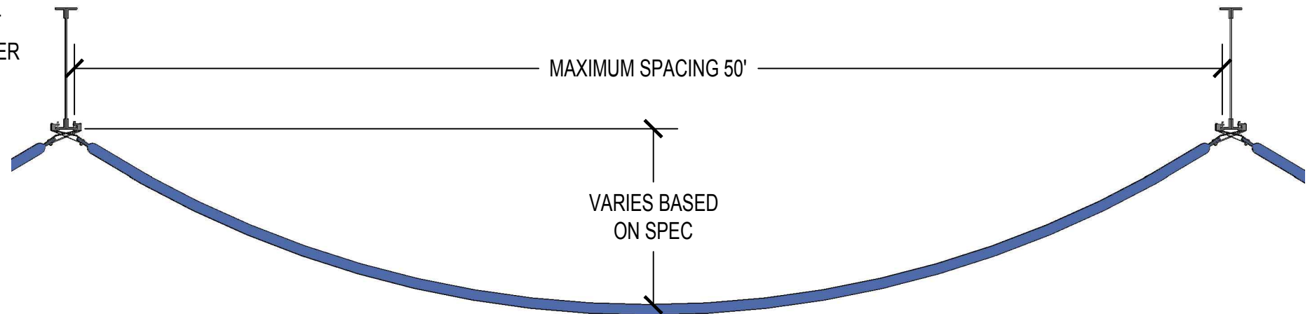
DROOP & BANNER LENGTH DETAIL
