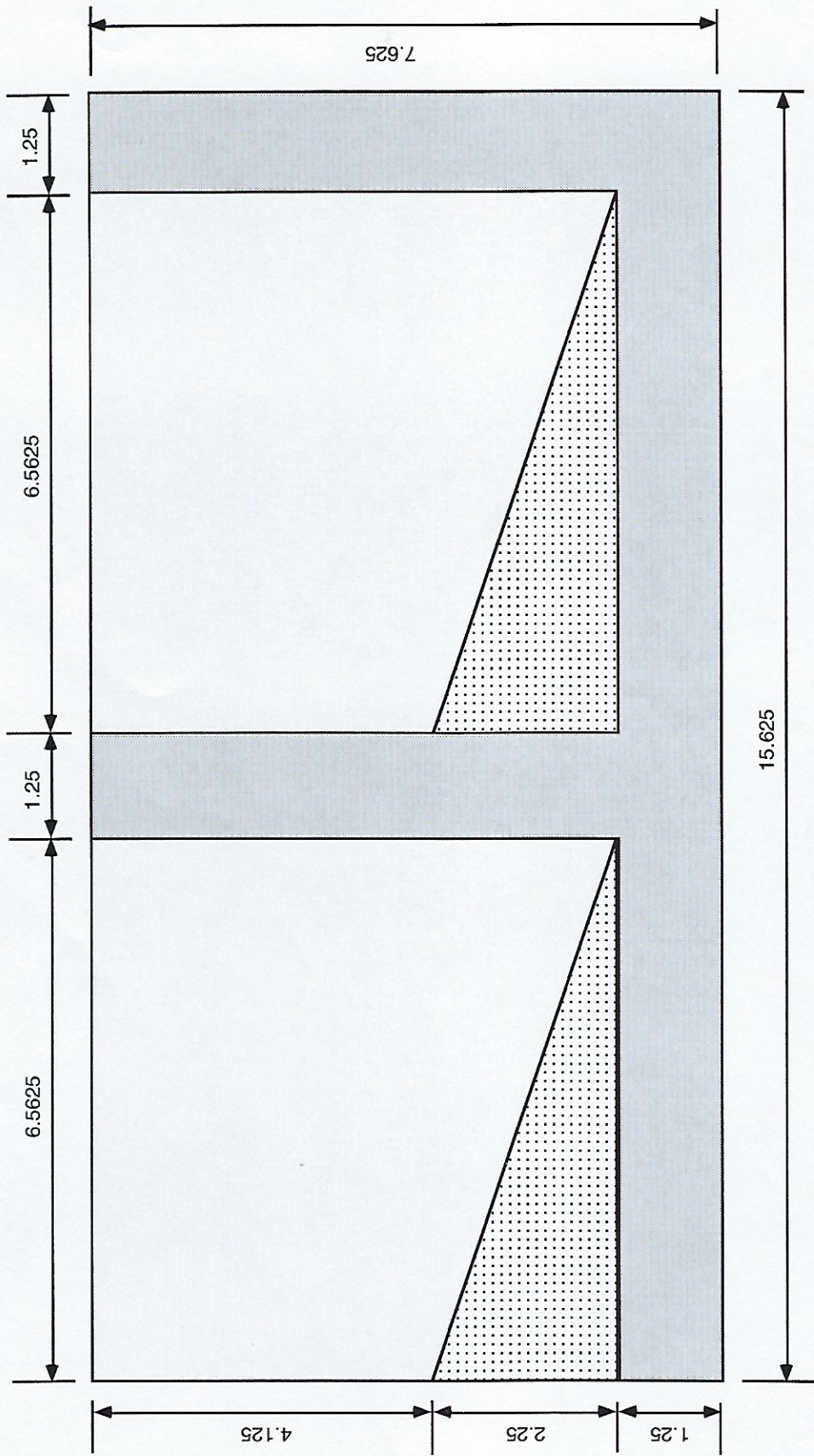
FRONT VIEW 8" & 12" SOUND CELL® SCALE: 1/2" = 1"
