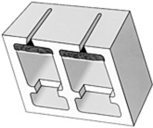
TYPE RSC (12")
