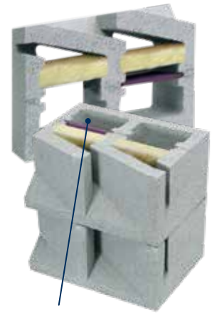
Optional Grout Shields (only available with 12" units as shown)
