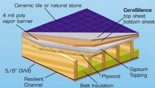
Typical Wood Construction
