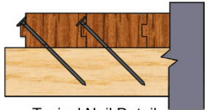
Typical Nail Detail
