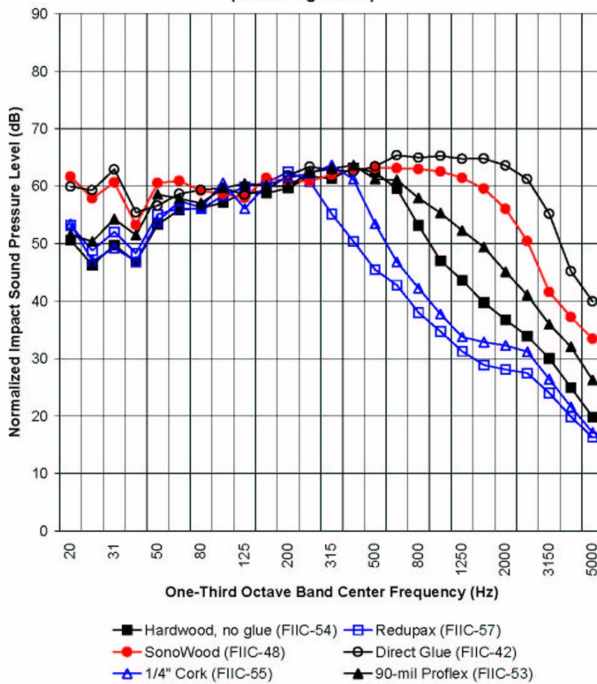
First & Clay Condos Impact Noise in Blakeley Garage Mockup Hardwood with various underlayments (no ceiling below)
